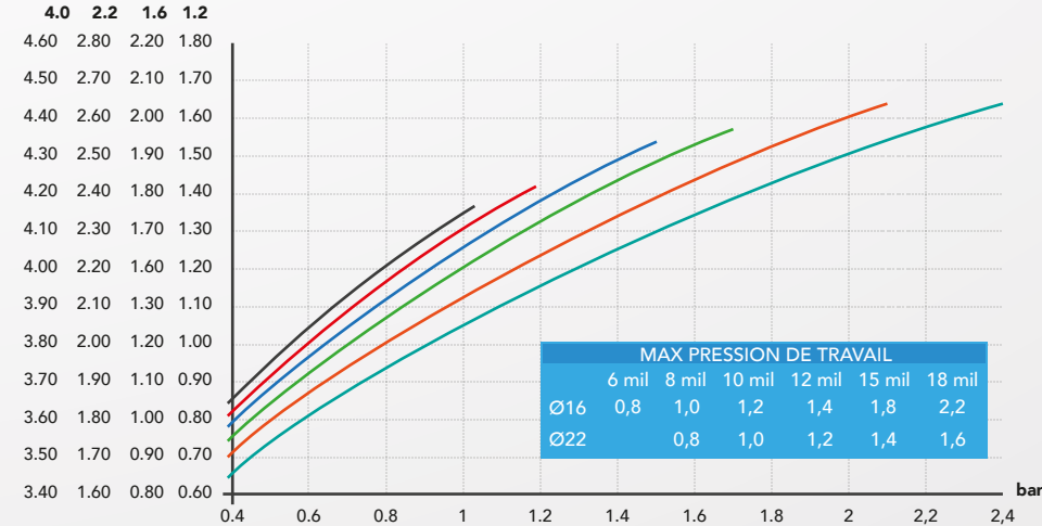
NOMINAL FLOW RATE (l/h) PORTATE (l/h)
